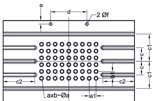
BOLSTER WITH DIE CUSHION
