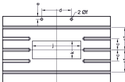
BOLSTER WITH RECTANGULAR OPENING
