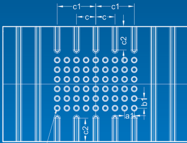
BOLSTER WITH DIE CUSHION
