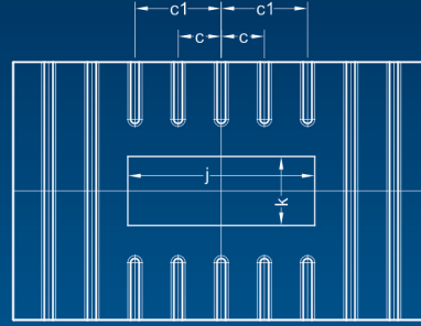
BOLSTER WITH RECTANGULAR OPENING
