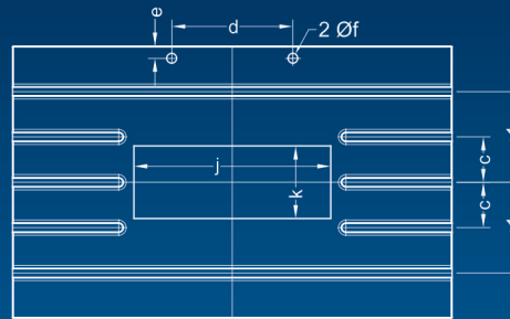
BOLSTER WITH RECTANGULAR OPENING
