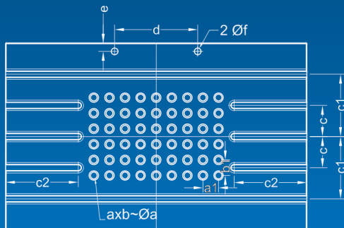
BOLSTER WITH DIE CUSHION
